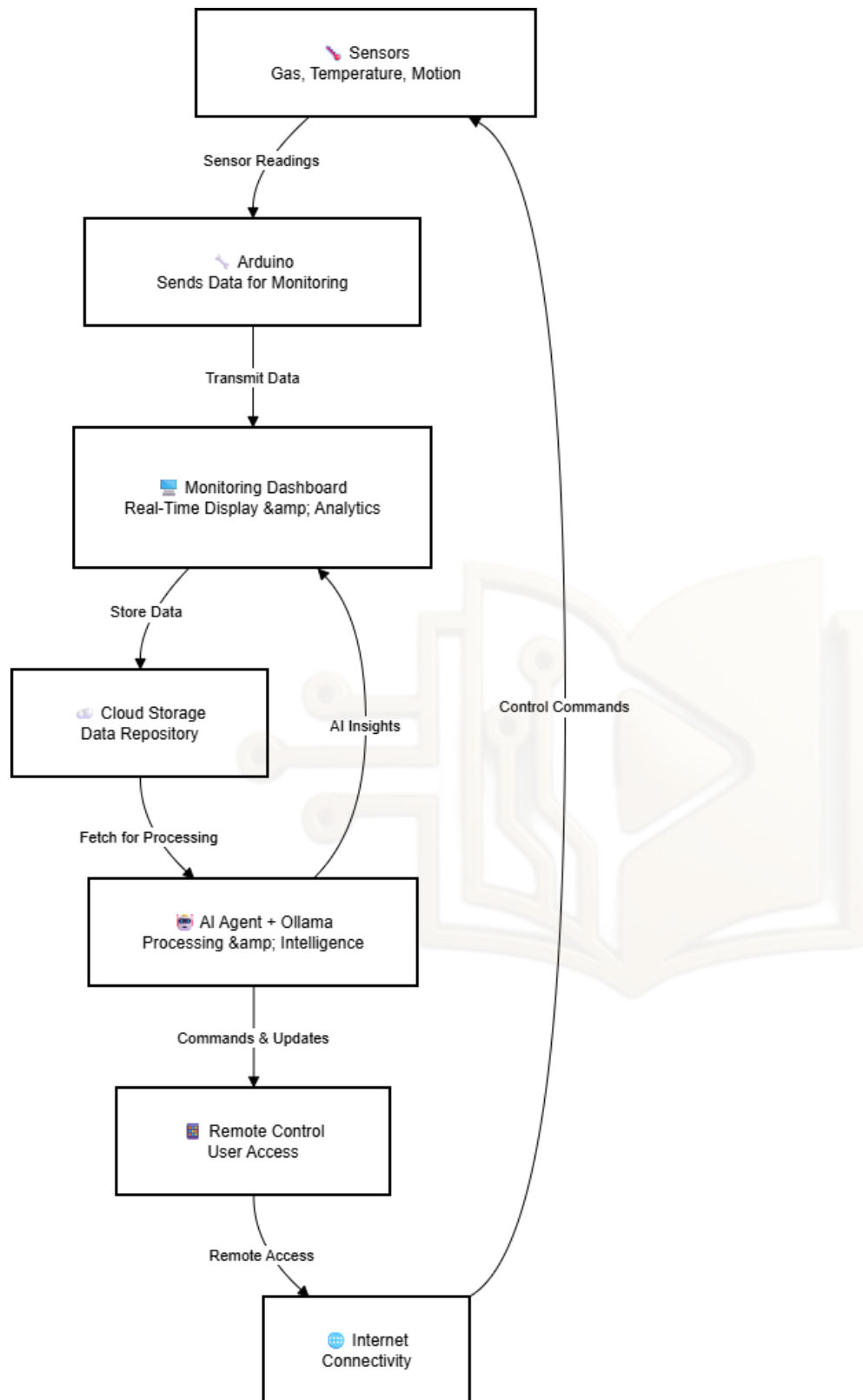
Figure: Data Flow Diagram for Smart Home Automation System
